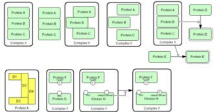
SuplFig5_StructureofComplex_3
